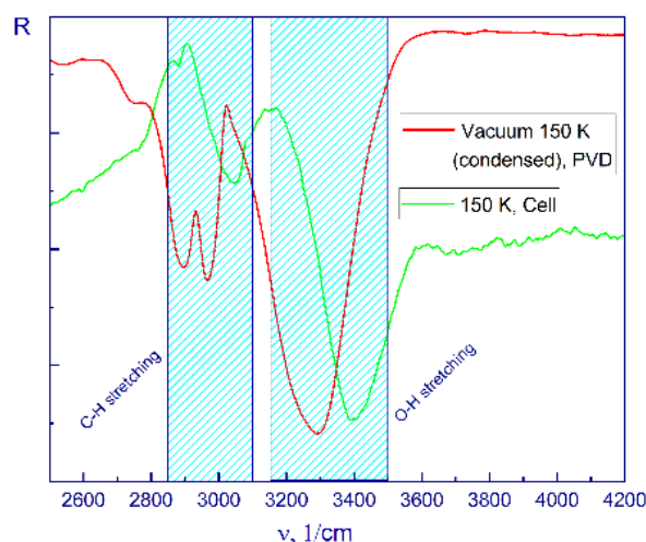
Figure 1 - Spectra of ethanol at 150 K from two experiments
