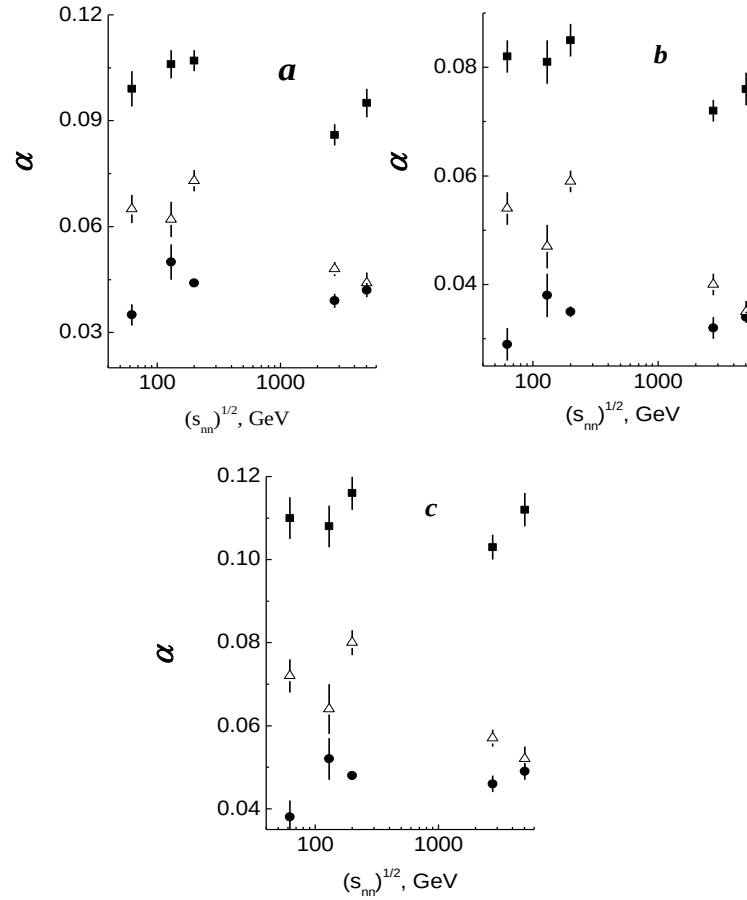
Figure 1 - The collision energy (s_{nn})^{1/2} dependencies of the power exponent parameter \alpha for the charged pions (●) and kaons ( \Delta ), protons and antiprotons (■), extracted from separate (independent) minimum \chi^2 fits of the experimental midrapidity \langle p_t \rangle versus \langle \frac{dN_{ch}}{d\eta} \rangle (a), \langle p_t \rangle versus \langle N_{coll} \rangle (b), and \langle p_t \rangle versus \langle N_{part} \rangle (c) dependencies of the charged pions and kaons, protons and antiprotons (in Au+Au collisions at (s_{nn})^{1/2}=62.4, 130 and 200 GeV, and in Pb+Pb collisions at (s_{nn})^{1/2}=2.76 and 5.02 TeV) by \langle p_t \rangle = C \cdot \langle \frac{dN_{ch}}{d\eta} \rangle^\alpha (Eq. (1)), \langle p_t \rangle = C \cdot \langle N_{coll} \rangle^\alpha (Eq. (2)), and \langle p_t \rangle = C \cdot \langle N_{part} \rangle^\alpha (Eq. (3)) function, respectively
